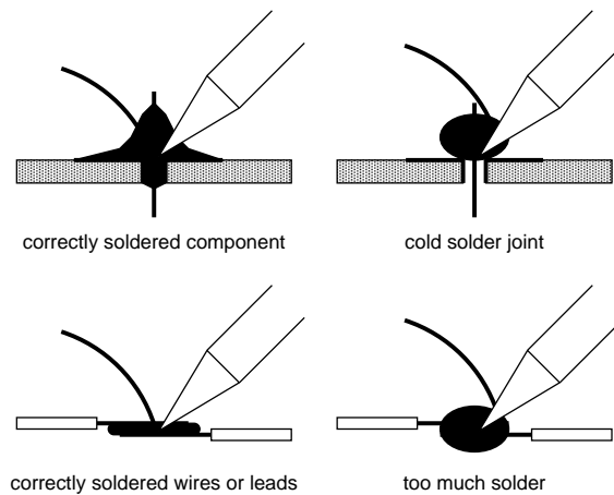
Figure 1: Soldering Joints
